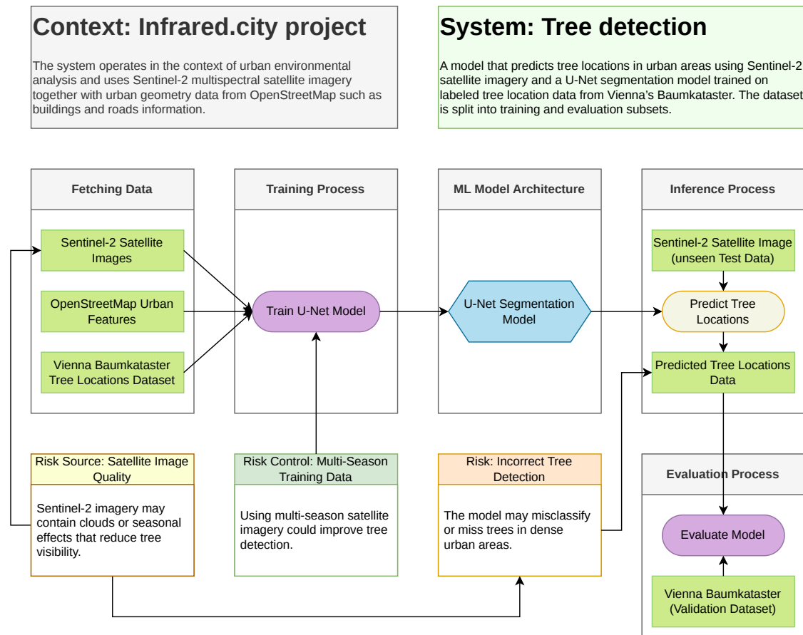
Figure 1: BEAM model of the proposed tree detection system.
